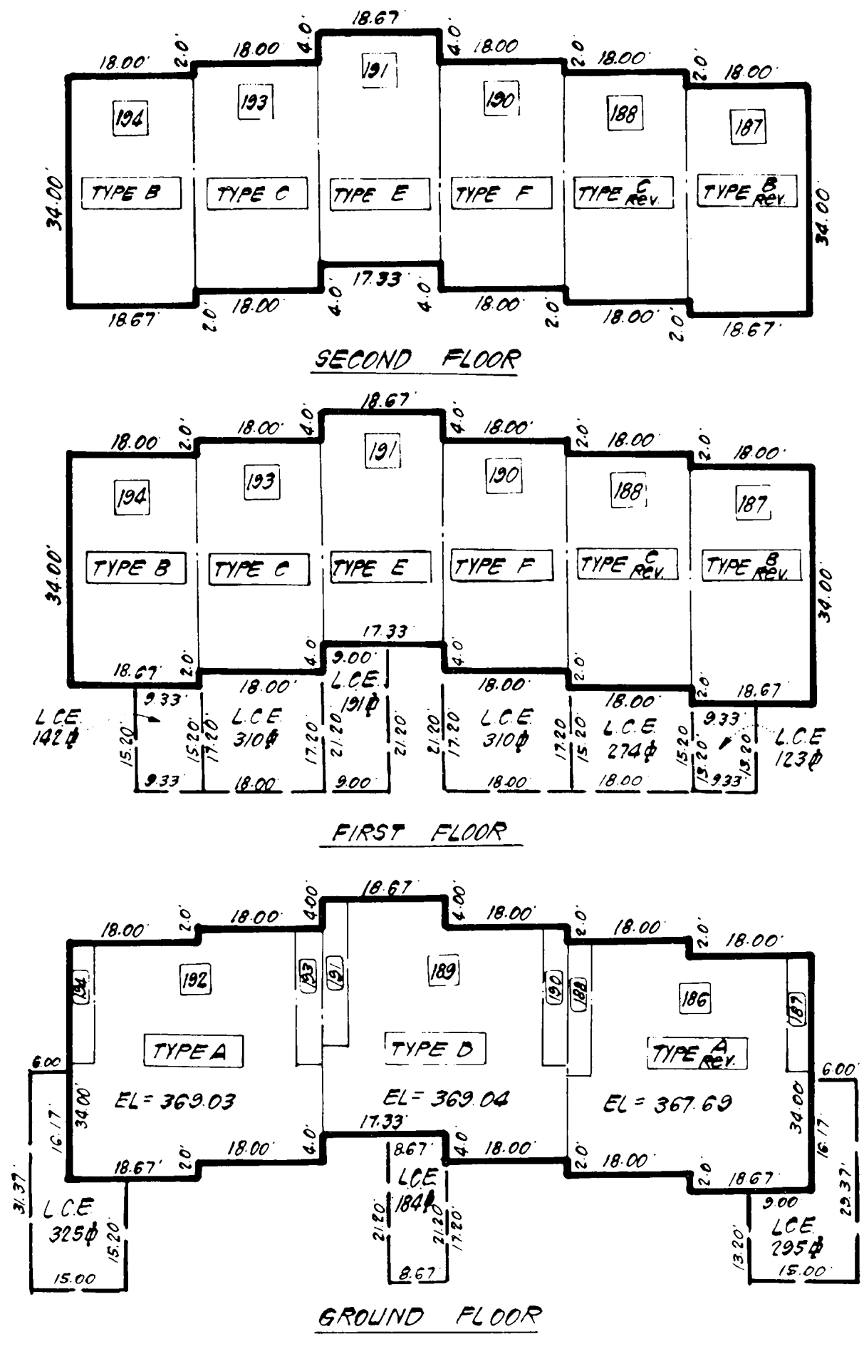
BUILDING NUMBER 26 SCALE: 1"=20'
